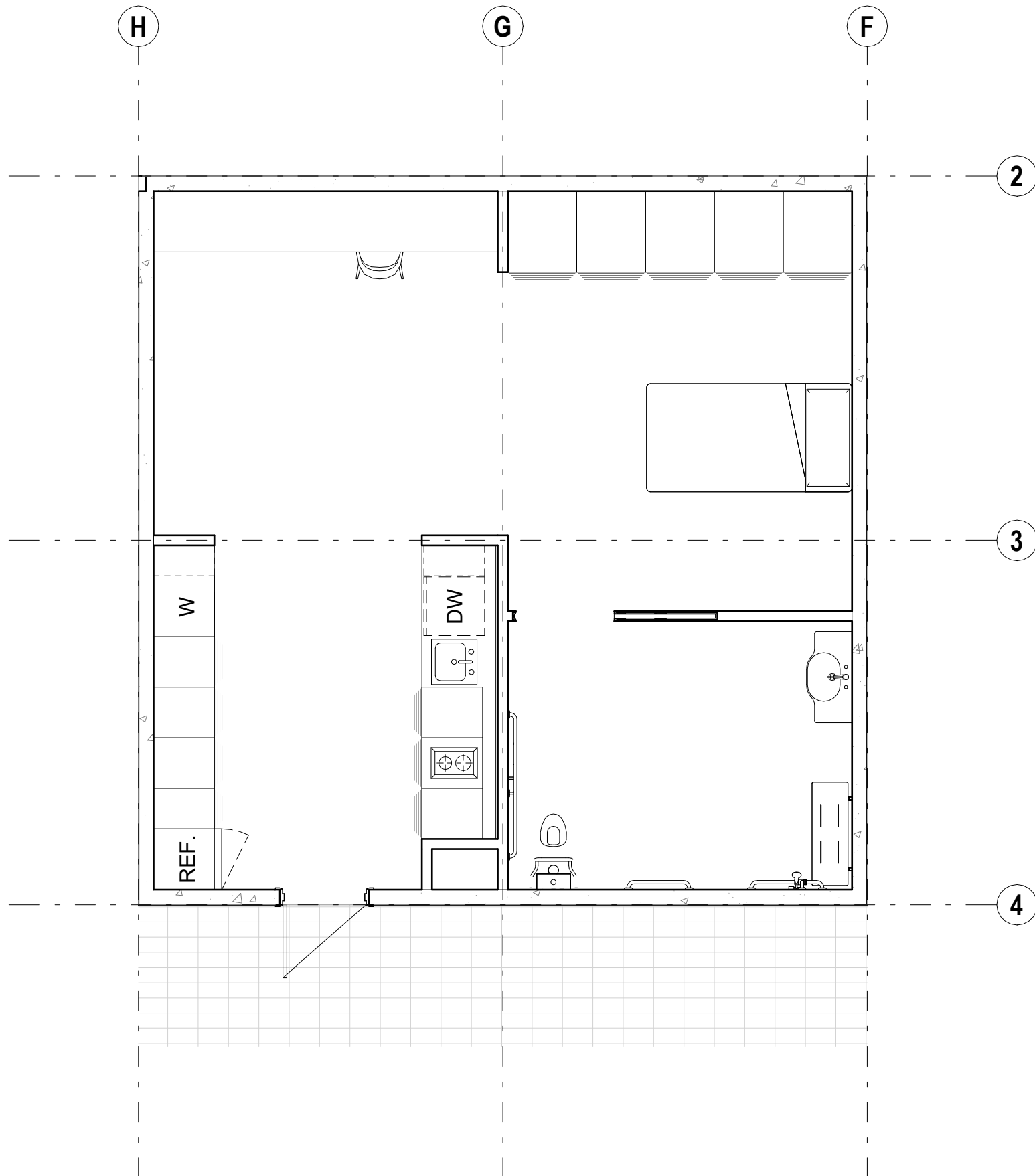
6 Unit Accessible Typology PLAN
