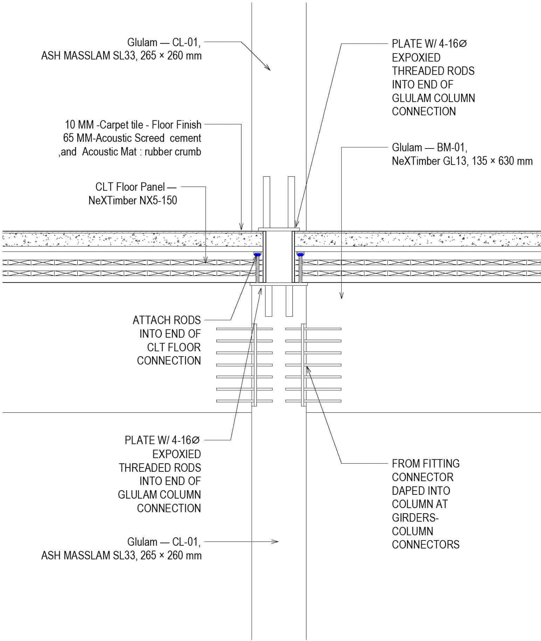
2 TYPICAL GIRDER - COLUMN CONNECTION 1 : 10
