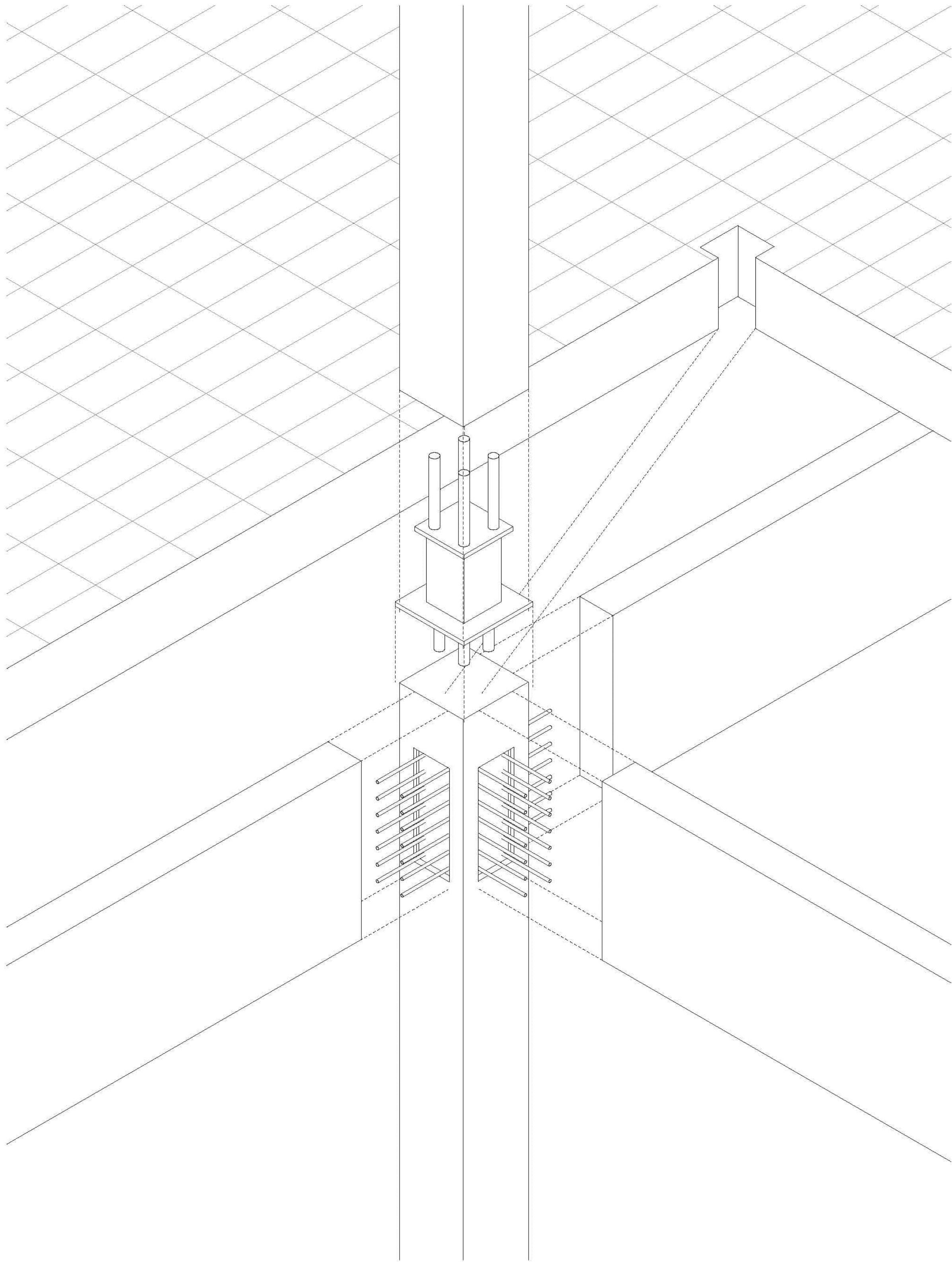
1 PROPOSED TYPICAL CONNECTION
