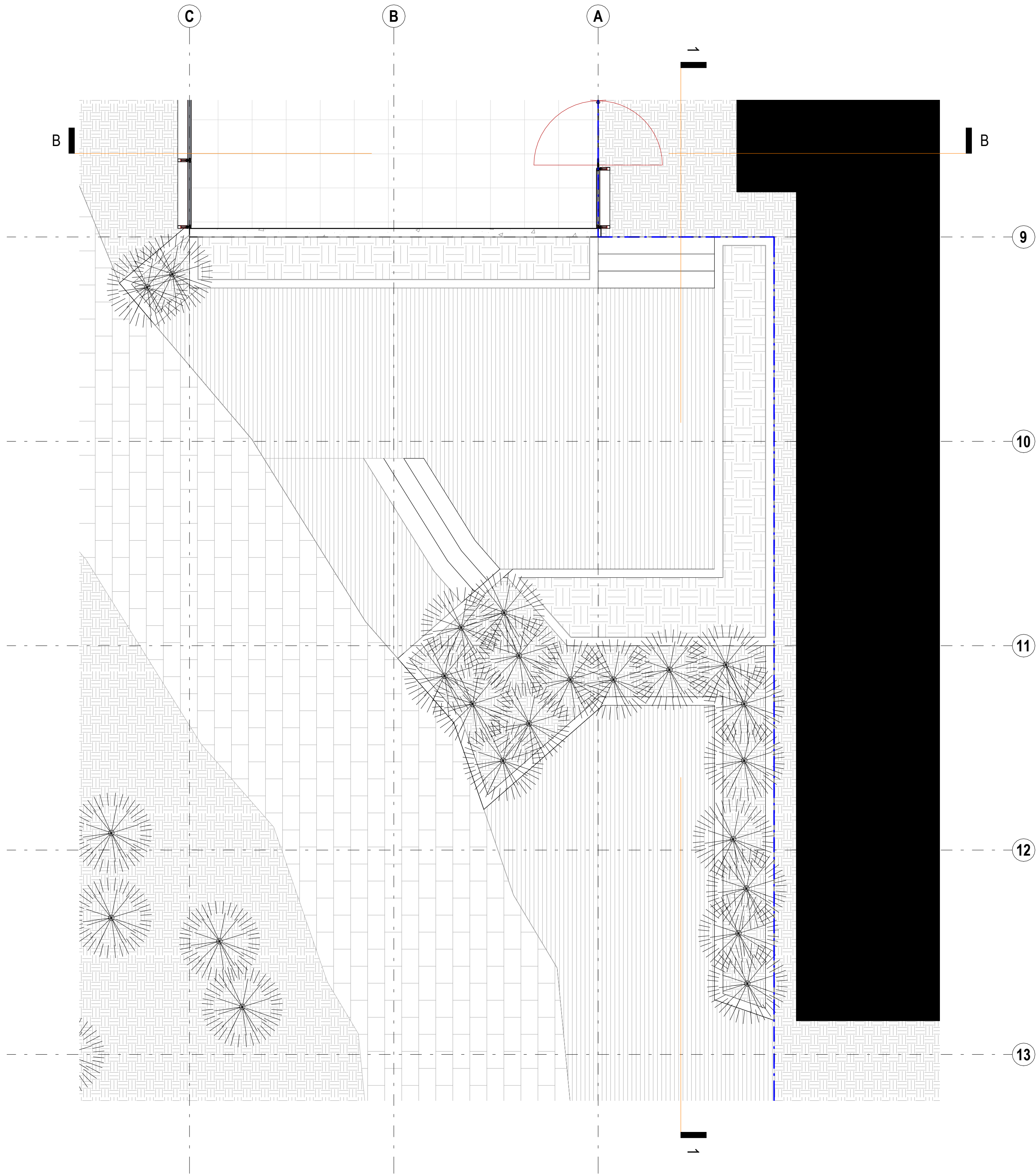
2 LEVEL 00 GROUND FLOOR PLAN - TIMBER DECK A403
